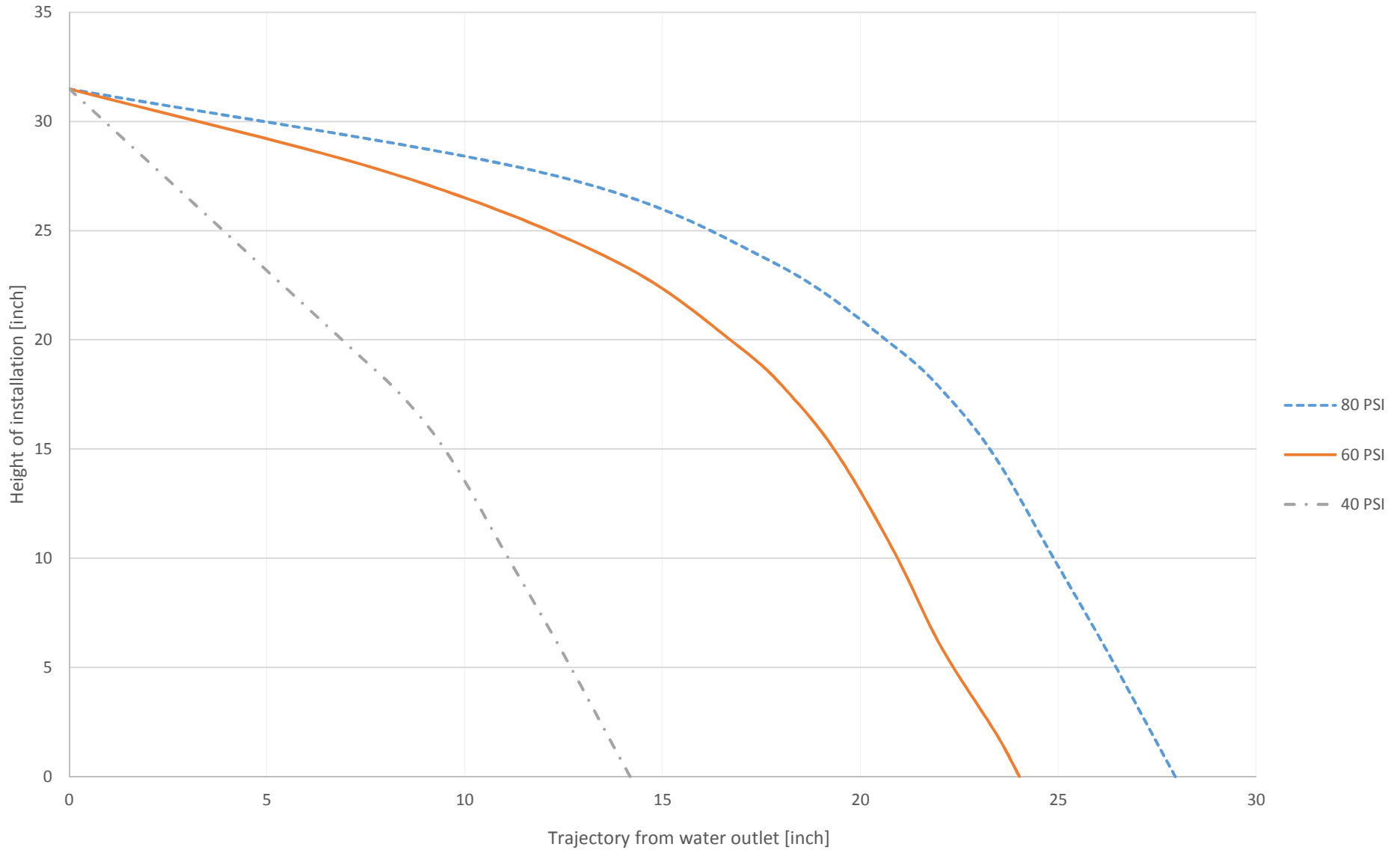
Trajectory length diagram G-8210 Height of installation 32"
