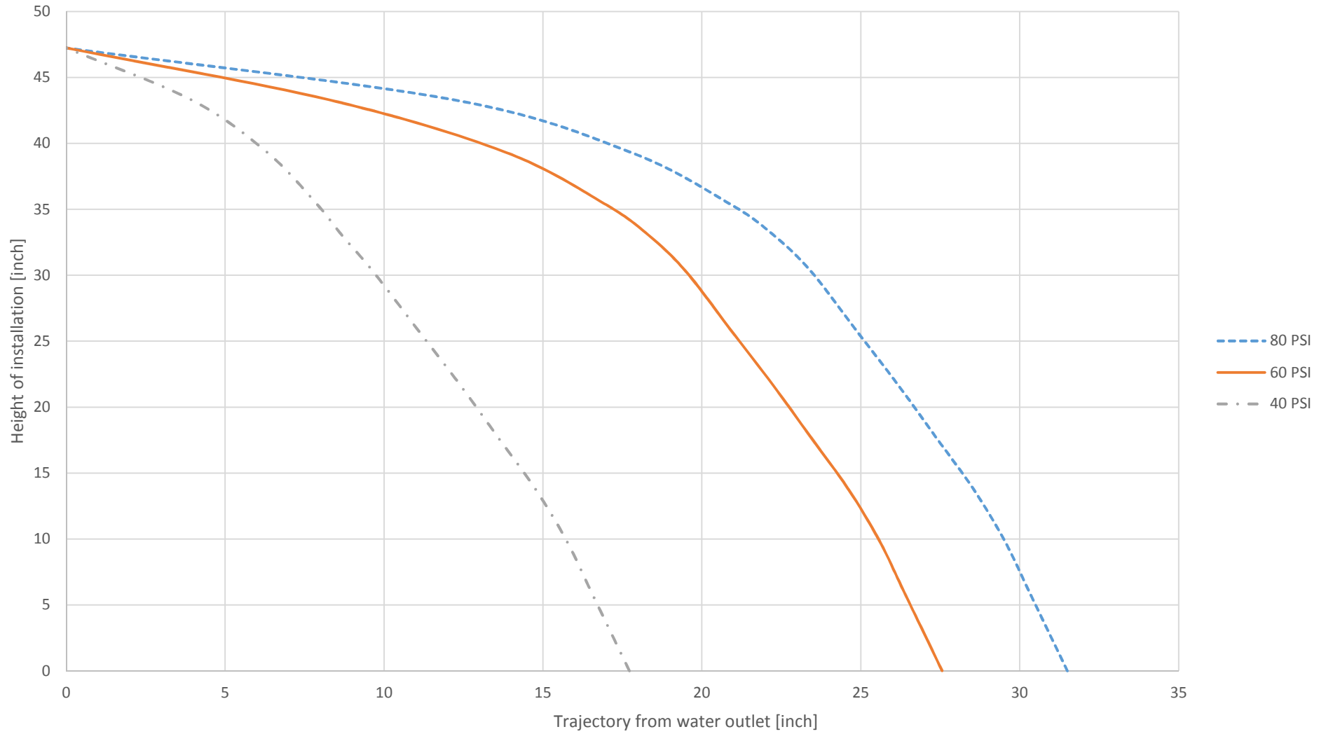
Trajectory length diagram G-8210 Height of installation 47"
